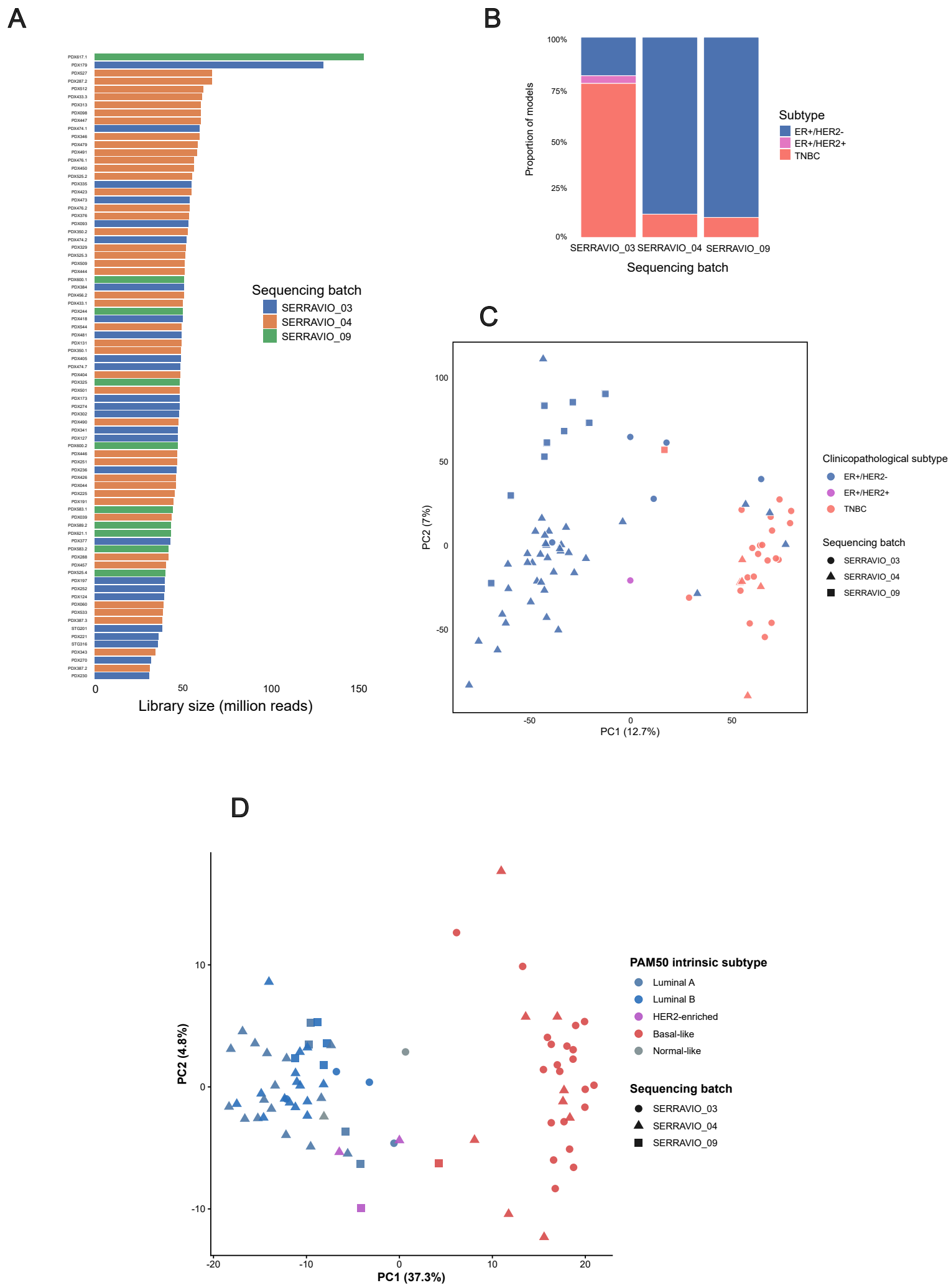
Supplementary Figure 1. QC and PAM50 subtype of baseline PDX bulk RNA-seq analysis
